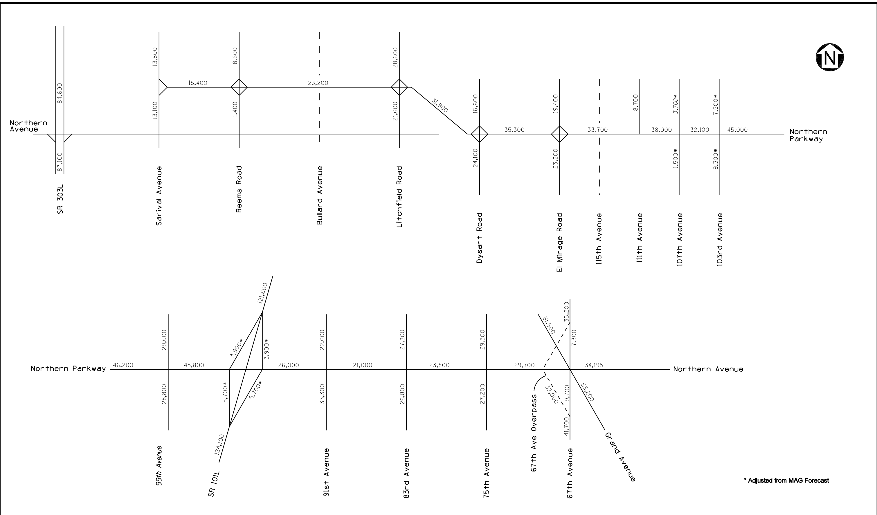
FIGURE 2-5 2015 WEST TO EAST WITHOUT LOOP 303 SYSTEM INTERCHANGE DAILY TRAFFIC PROJECTIONS
